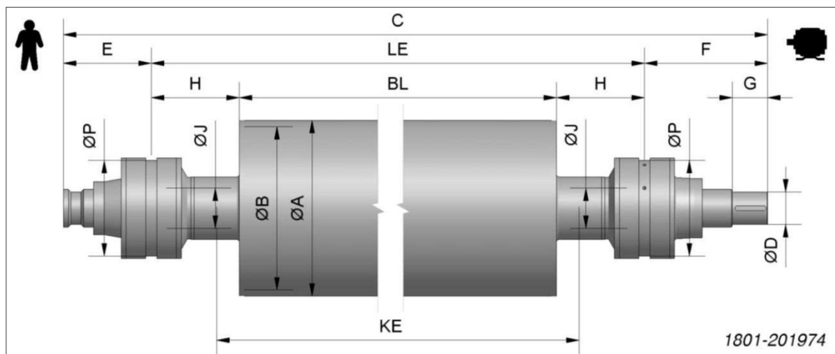
Fig. 3-2 Component specifications
